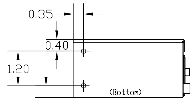
DMP200 MOUNTING TRAY LEFT SIDE
