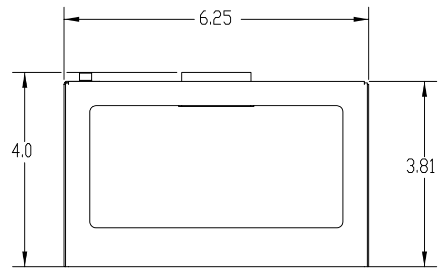
DMP200 MOUNTING TRAY TOP VIEW
