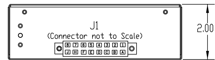
DMP200 MOUNTING TRAY FRONT VIEW
